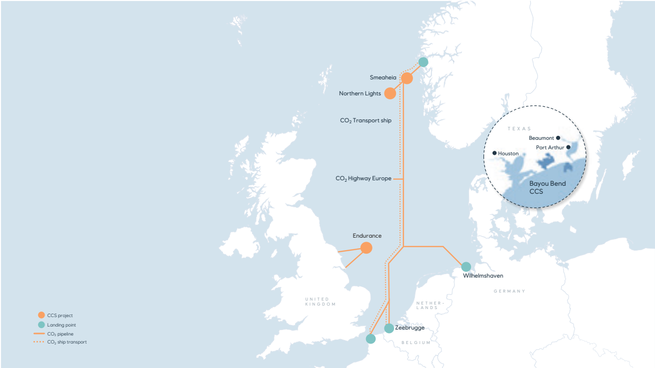
FIGURE 36 CO 2 HIGHWAY EUROPE AND NORWAY-GERMANY PIPELINE
