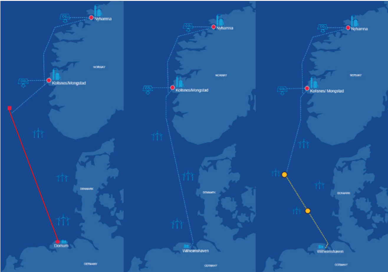
Concept 1: Europe re-purpose Concept 2: New pipeline to WHV Concept 3: Tie-in to AquaDuctus
