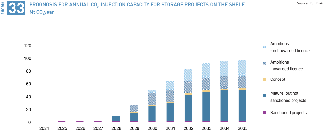
Figure 33. Forecast of annual CO 2 injection capacity for storage projects on the continental shelf with varying degrees of maturity (Mt CO 2 /year). The graph shows the expected future cumulative injection capacity in storage projects planning to commence injection before the year on the x-axis. Note that storage projects typically scale up injection over time as they contract and receive CO 2 from multiple customers. Commencing injection in a particular year therefore does not imply reaching full injection capacity in the same year.
